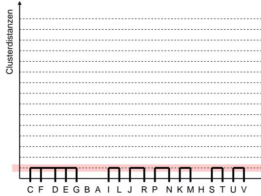
Dendrogram (Single Link)
