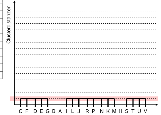
Dendrogram (Single Link)
