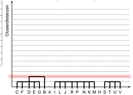
Dendrogram (Single Link)
