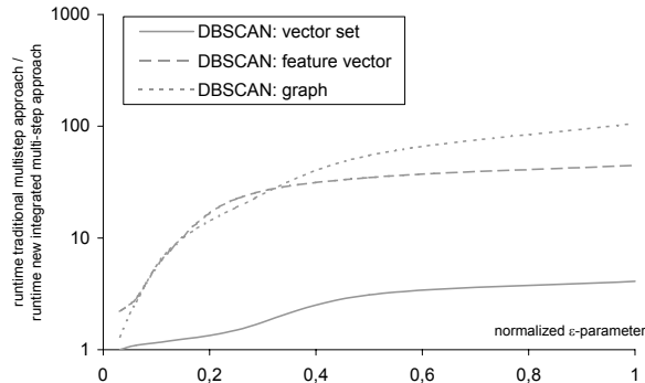
Fig. 8. Speed-up dependent on the \epsilon -parameter.
