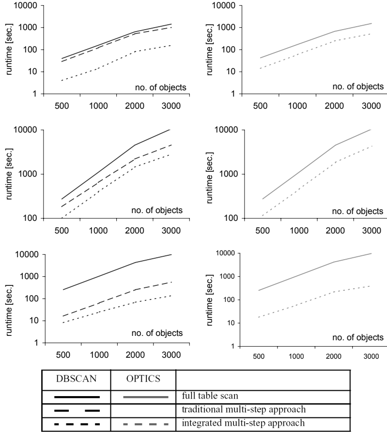
Fig. 9. Absolute runtimes w.r.t. varying database sizes.
