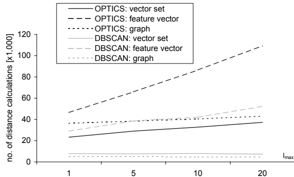
Fig. 10. Distance calculations for approximated clusterings.
