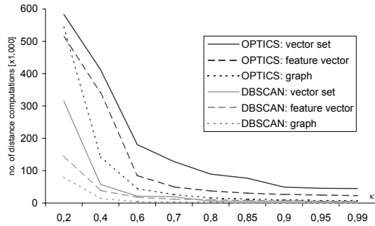
(a) Dependency on the filter quality d_f(o_1, o_2) = \kappa \cdot d_o(o_1, o_2) .
