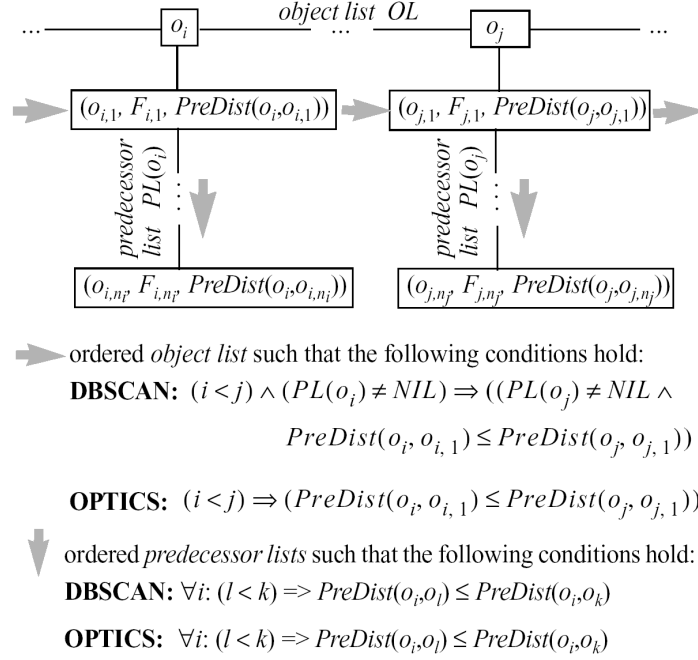
Fig. 5. Data structure Xseedlist.
