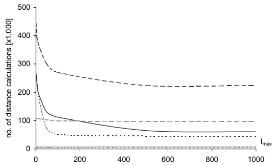
(c) Dependency on the maximum allowed length of the predecessor lists.
