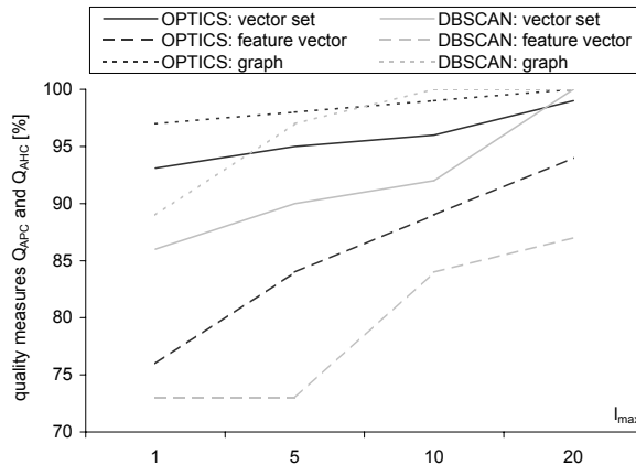
Fig. 11. Quality measures for approximated clusterings.
