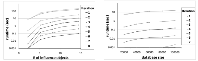
(a) Runtime w.r.t. number of influence objects.
