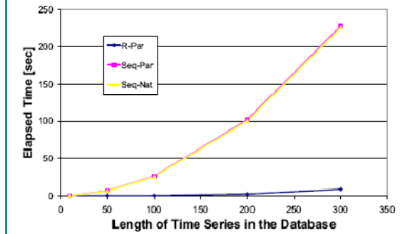
(b) Scalability against time series length.
