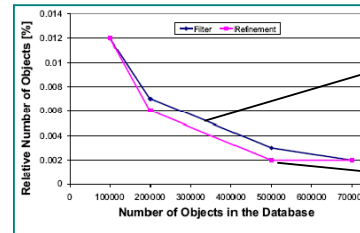
(a) Pruning power for varying database size.
