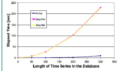
(b) Scalability against time series length.
