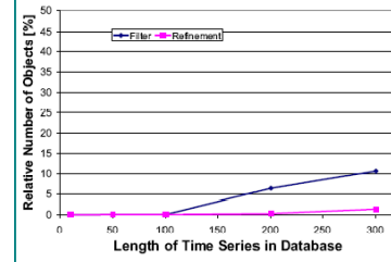
(b) Pruning power for varying time series length.
