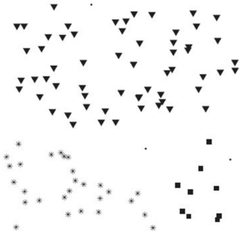
DBSCAN (3 Cluster)
