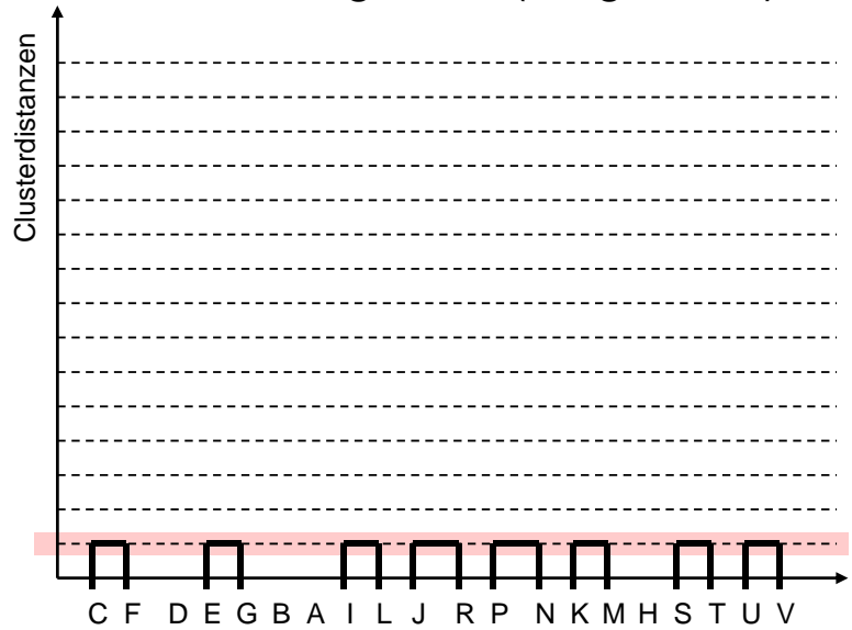
Dendrogramm (Single Link)
