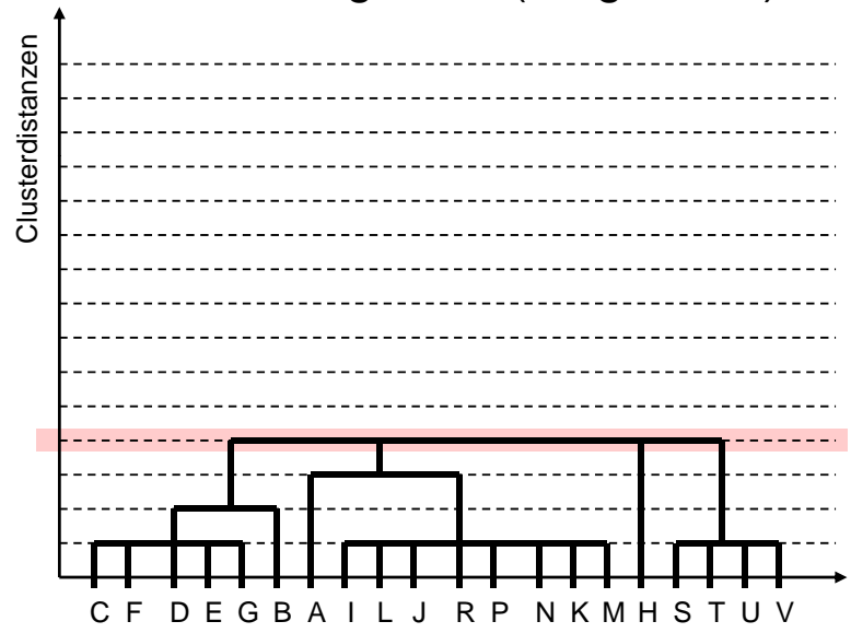
Dendrogramm (Single Link)
