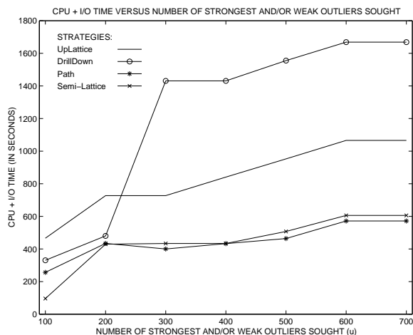
Figure 8: Top- u Strongest and/or Weak Outliers
