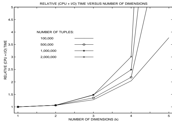
Figure 5: Heuristic Selection of k for JumpLattice
