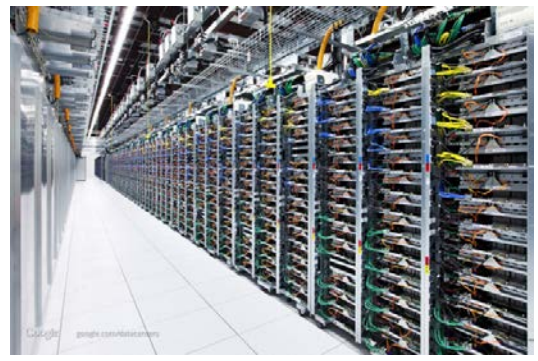
Racks of servers (and switches at the top), at Google's Mayes County, Oklahoma data center [extremetech.com]
