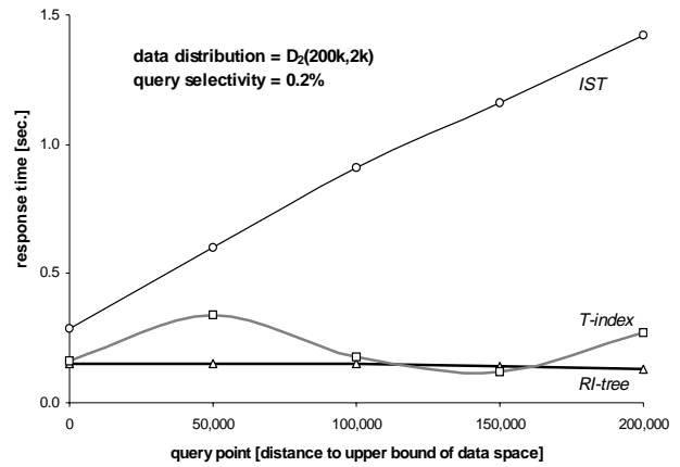
Figure 17: Response time for a “sweeping” point query on a D_2 data distribution. The IST degenerates with higher distance to the upper bound of the data space.
